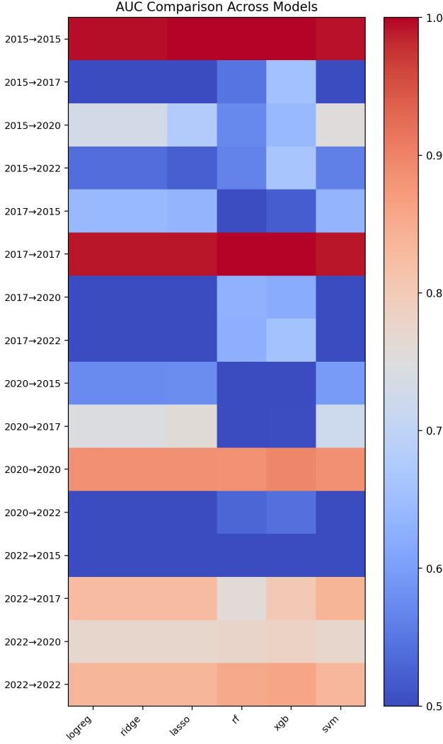
Figure 5: Cross-era AUC Comparison Across Models
